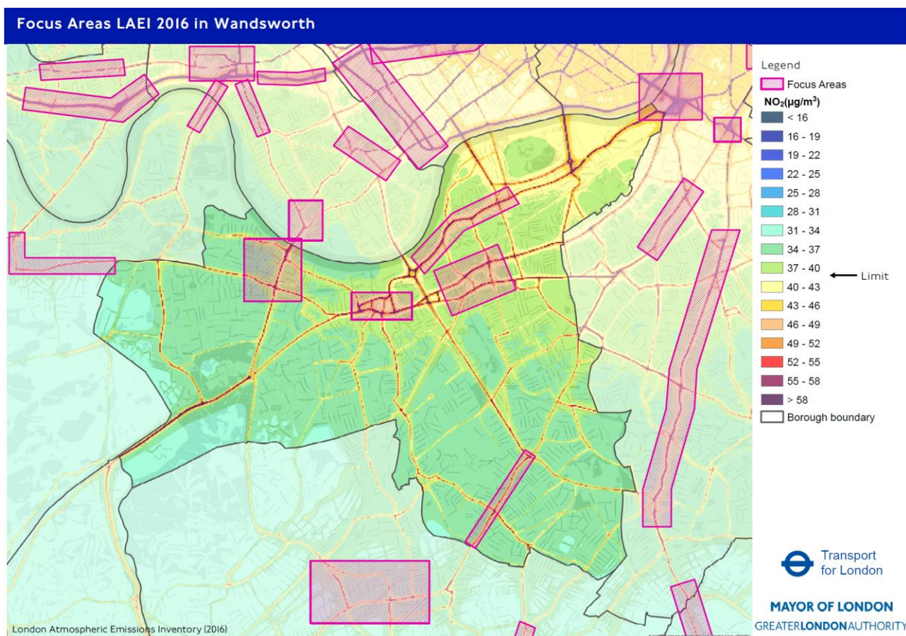
Figure 7 LB Wandsworth Focus Areas, London Atmospheric Emissions Inventory (LAEI 2016)
