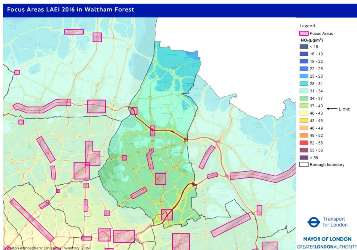
Figure 7 LB Waltham Forest Focus Areas, London Atmospheric Emissions Inventory (LAEI 2016)
