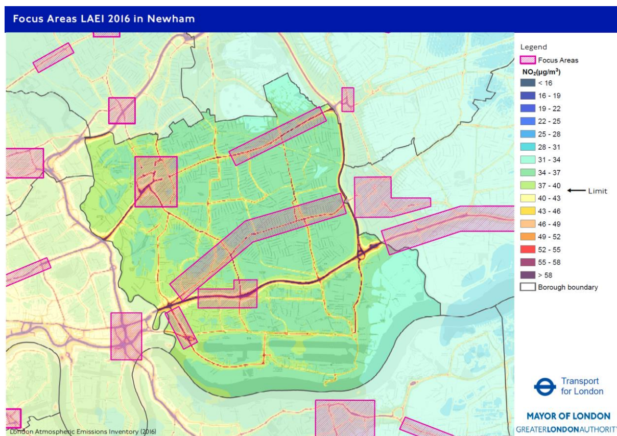
Figure 7 LB Newham Focus Areas, London Atmospheric Emissions Inventory (LAEI 2016)
