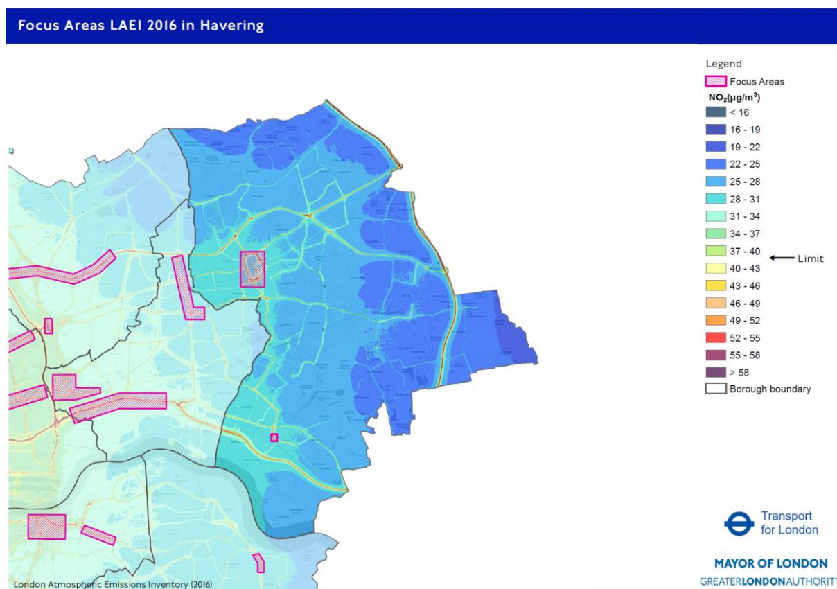
Figure 7 LB Havering Focus Areas, London Atmospheric Emissions Inventory (LAEI 2016)
