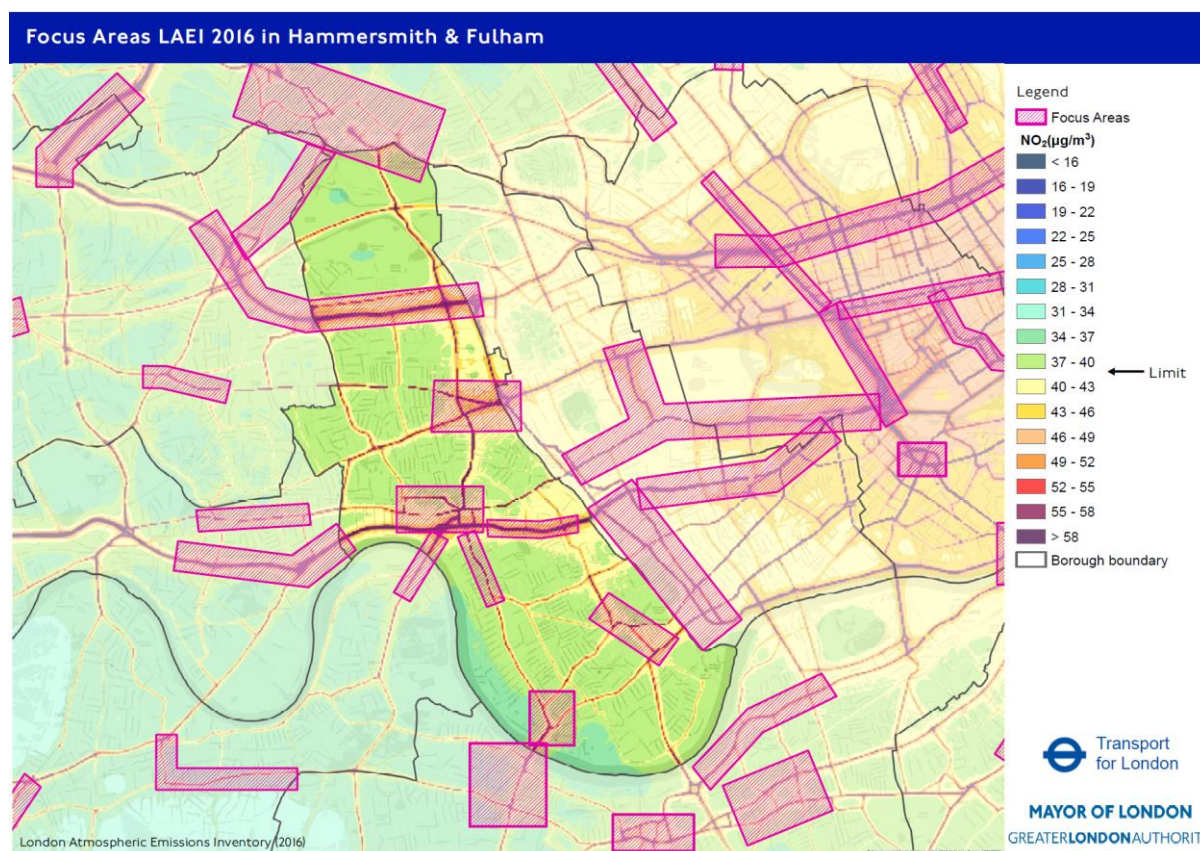
Figure 7 LB Hammersmith and Fulham Focus Areas, London Atmospheric Emissions Inventory (LAEI 2016)
