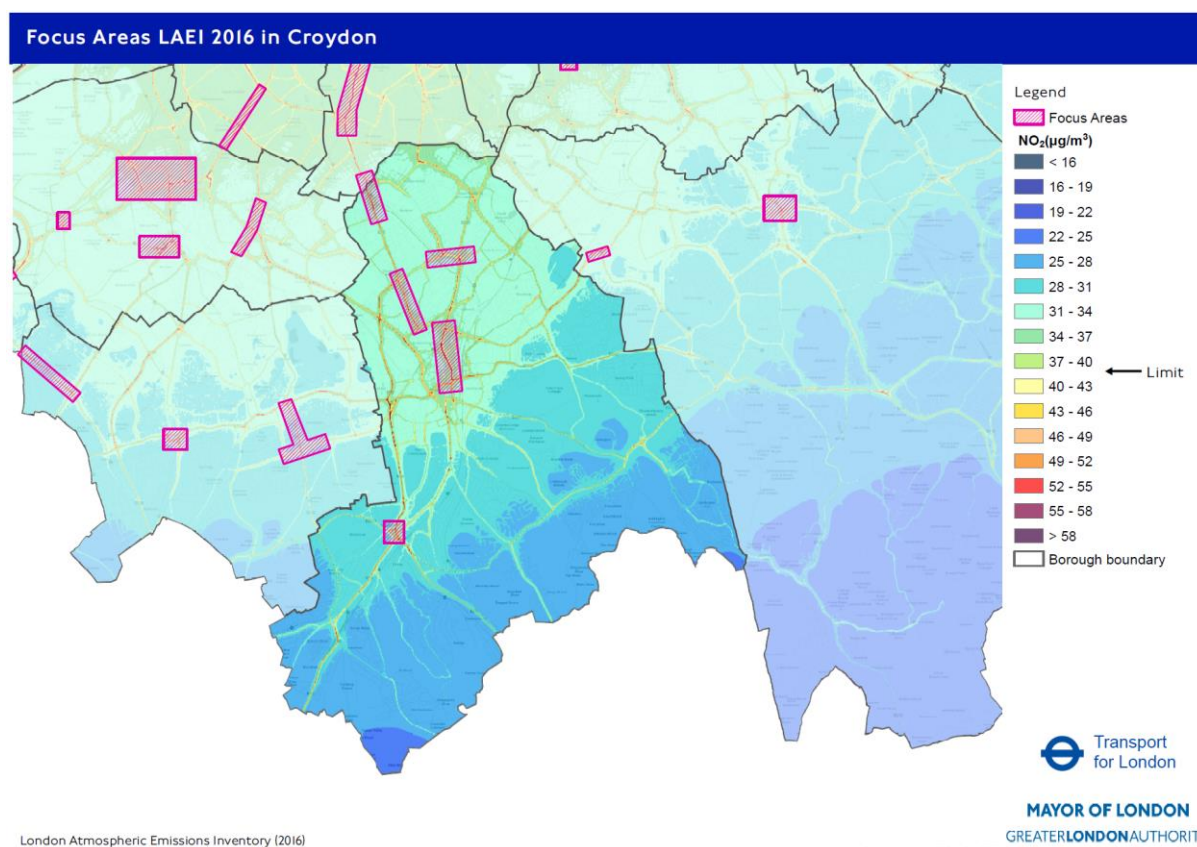
Figure 7 LB Croydon Focus Areas, London Atmospheric Emissions Inventory (LAEI 2016)
