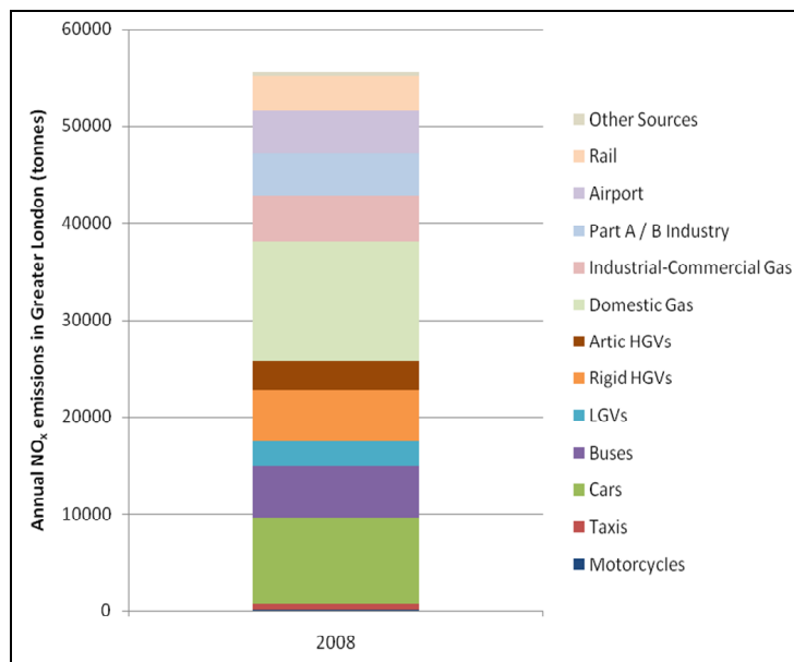
Image 2: NO x emissions from all direct sources in Greater London in 2008 (from Mayor's Air Quality Strategy MAQS) 3
