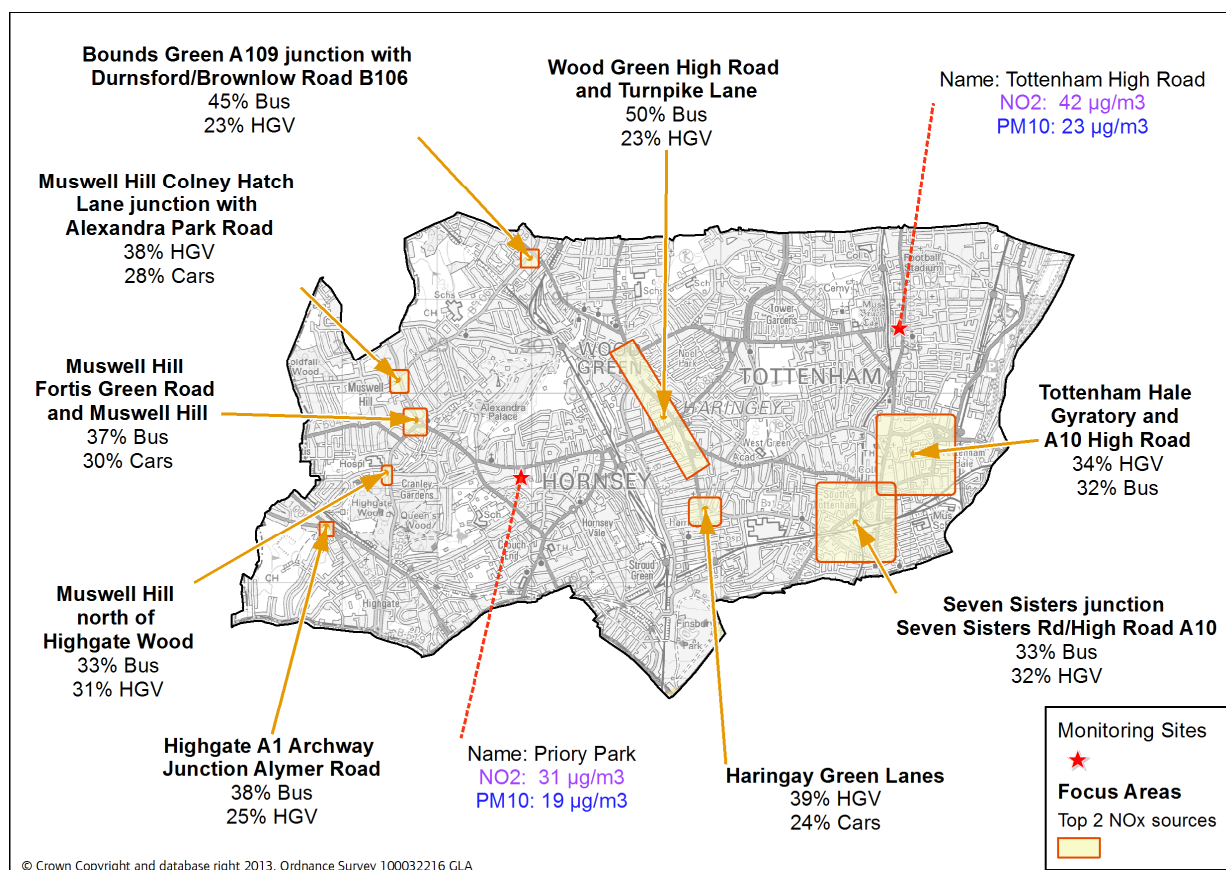
Image 4 – TfL NO 2 Focus Areas with Air Quality Monitoring locations.
