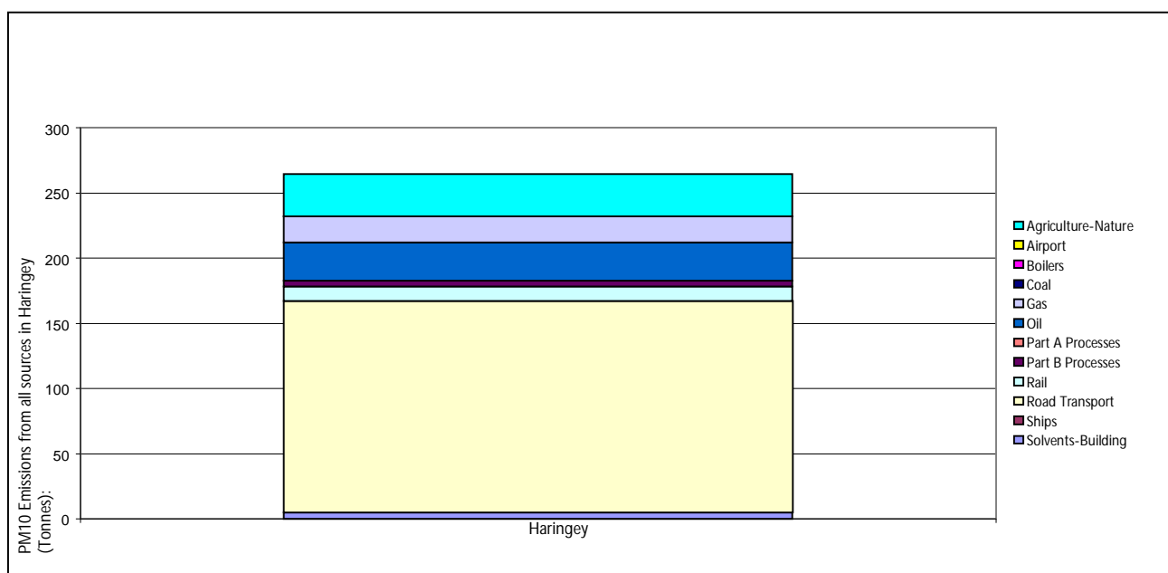
Image 3: Emission source contributions in LB Haringey (LAEI)
