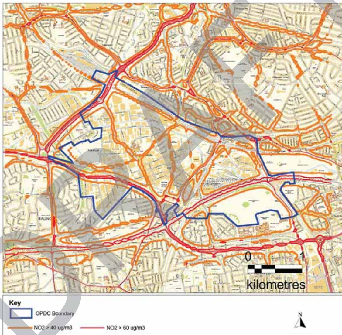
Figure 3.4 Contour map displaying LAEI NO 2 mapped concentrations
