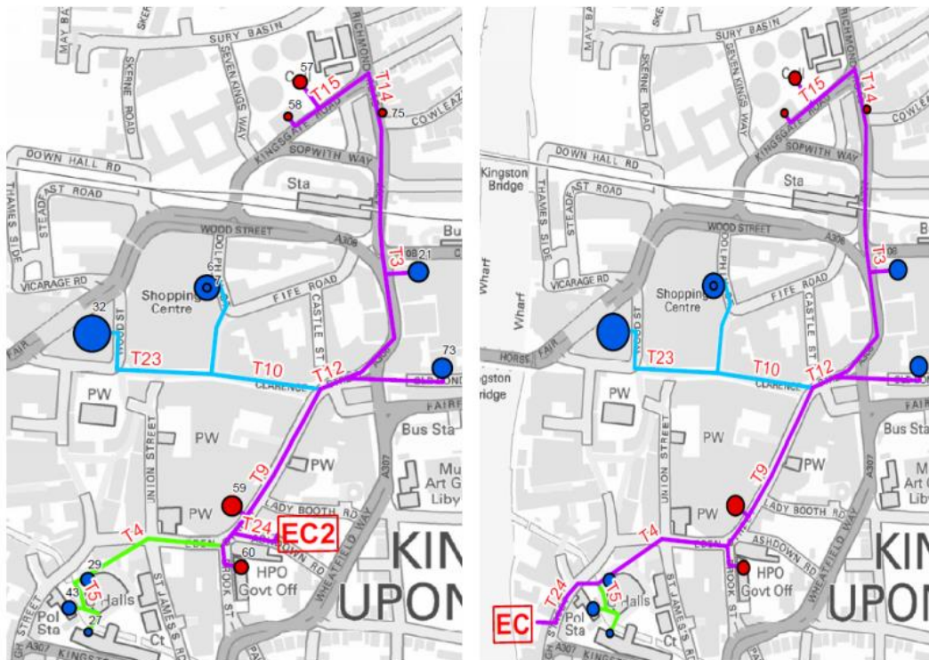
Figure 14 The CHP supply option located at Ashdown Road Car Park (left) and the WSHP supply option located at Eagle Brewery Wharf (right)
