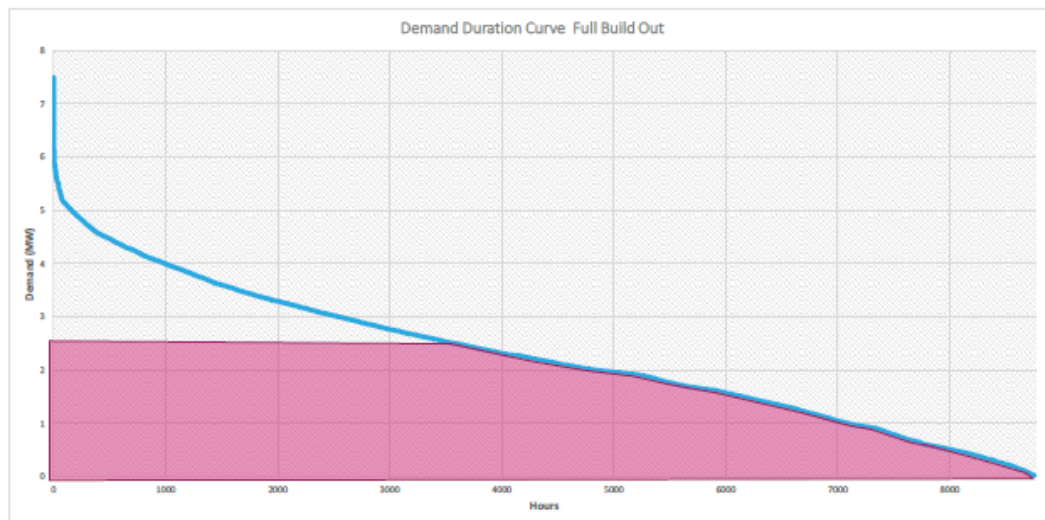
Figure 25 Kingston Town Centre heat demand and WSHP installed capacity
