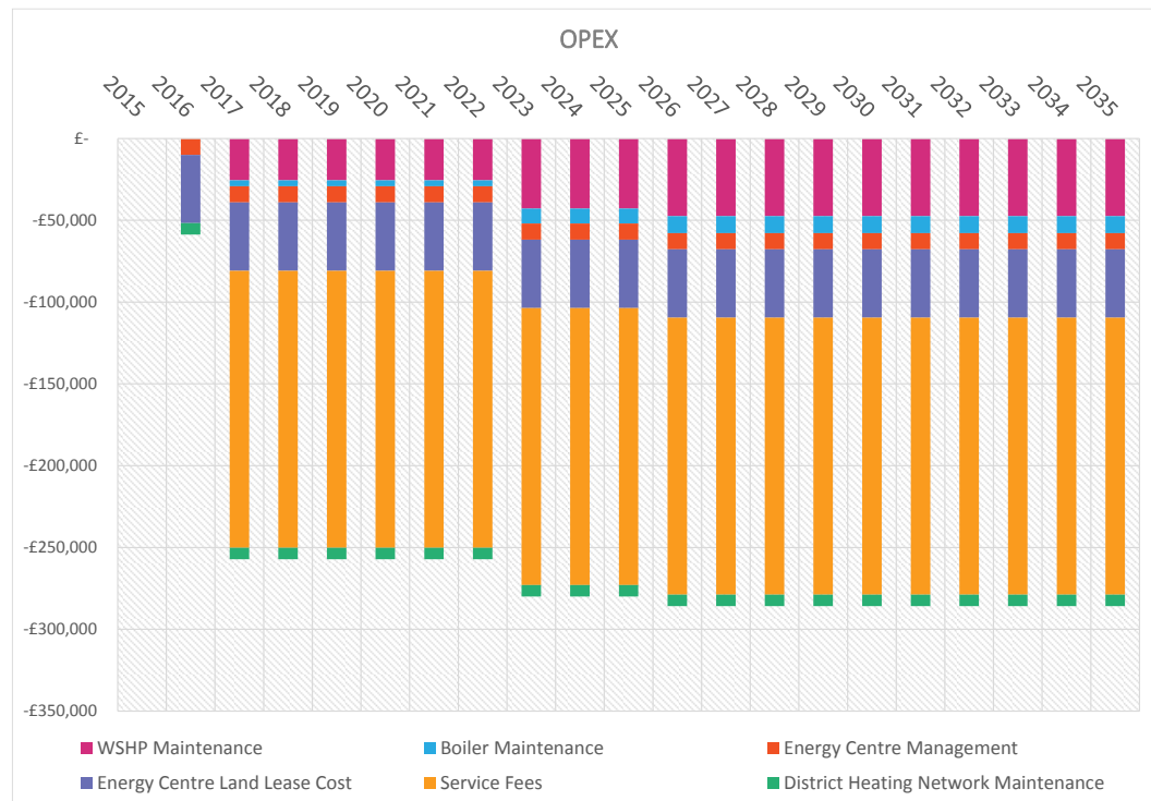
Figure 27 Operational costs of the Kingston Town Centre WSHP DH network
