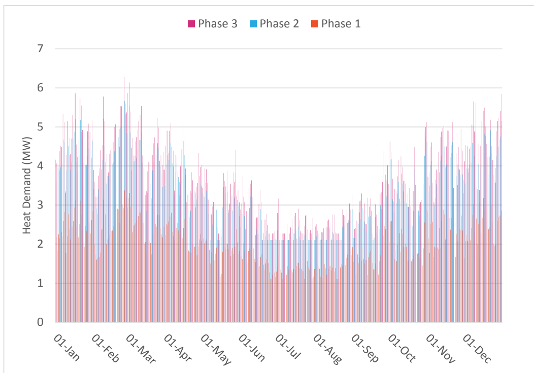
Figure 51 - Hourly heat demand profiles for the Kingston Town Centre network for all 3 phases
