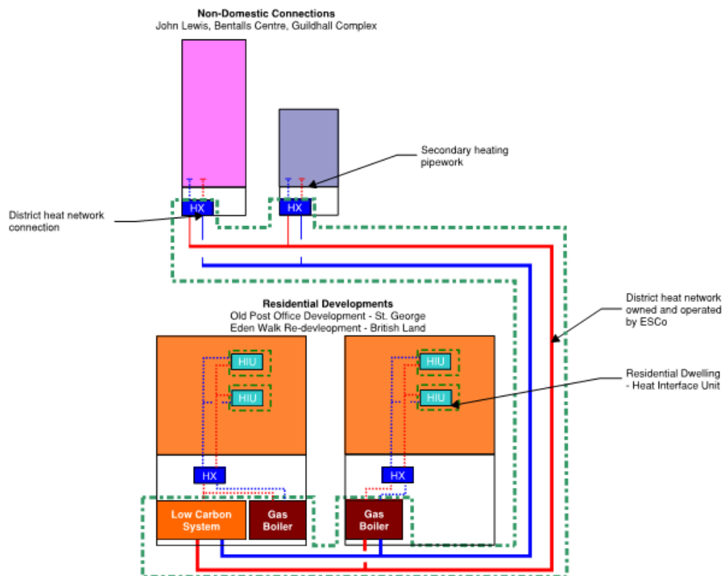
Figure 45 Alternative DH network configuration with a split energy centre
