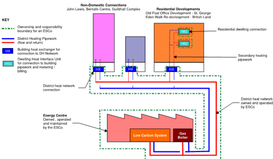
Figure 44 District heating network configuration and ownership
