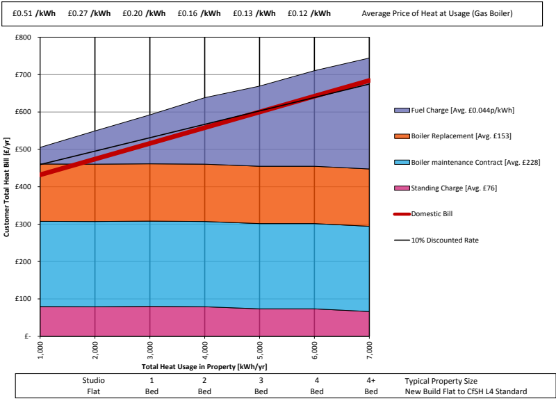
Figure 19 Price of heat for individual gas fired boilers and comparison to proposed Kingston DH network tariff (red line)
