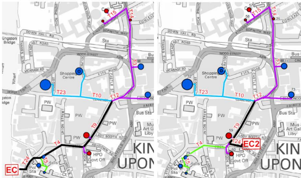
Figure 12 Future proofed elements (indicated in black) of the Kingston Town Centre DH network. WSHP energy centre (left) and CHP energy centre (right).
