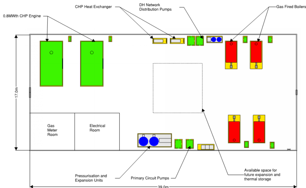
Figure 8 Preliminary CHP supply option energy centre layout
