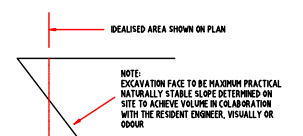
EXCAVATION DETAIL 1
