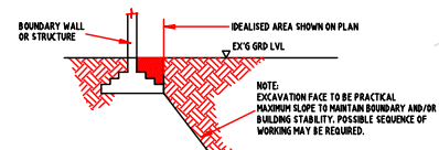
BOUNDARY/BUILDING ZONAL EXCAVATION DETAIL 2
