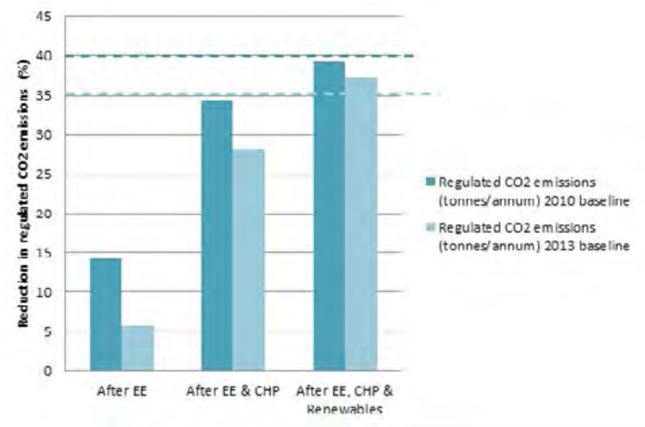
FIGURE 3 CO 2 EMISSIONS
