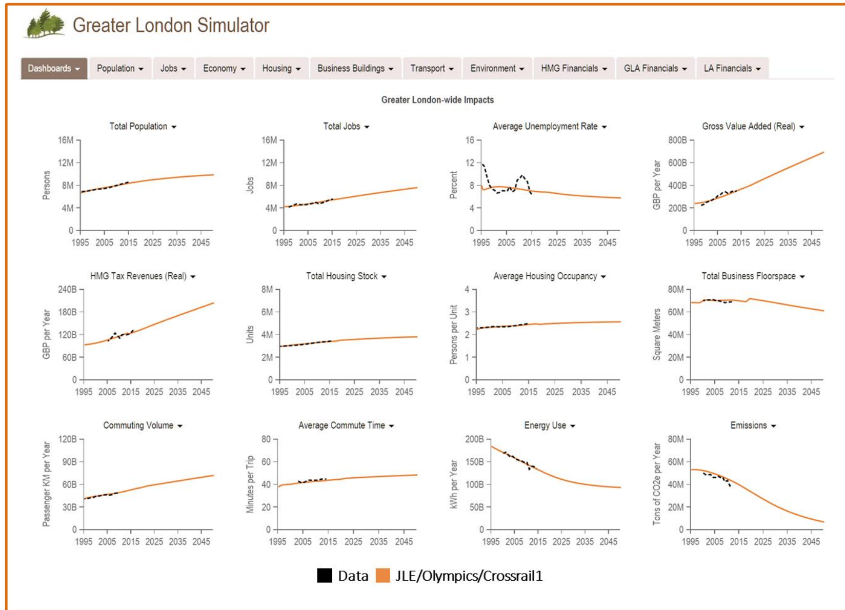
Figure 15 – Greater London Simulator recreating London's recent history
