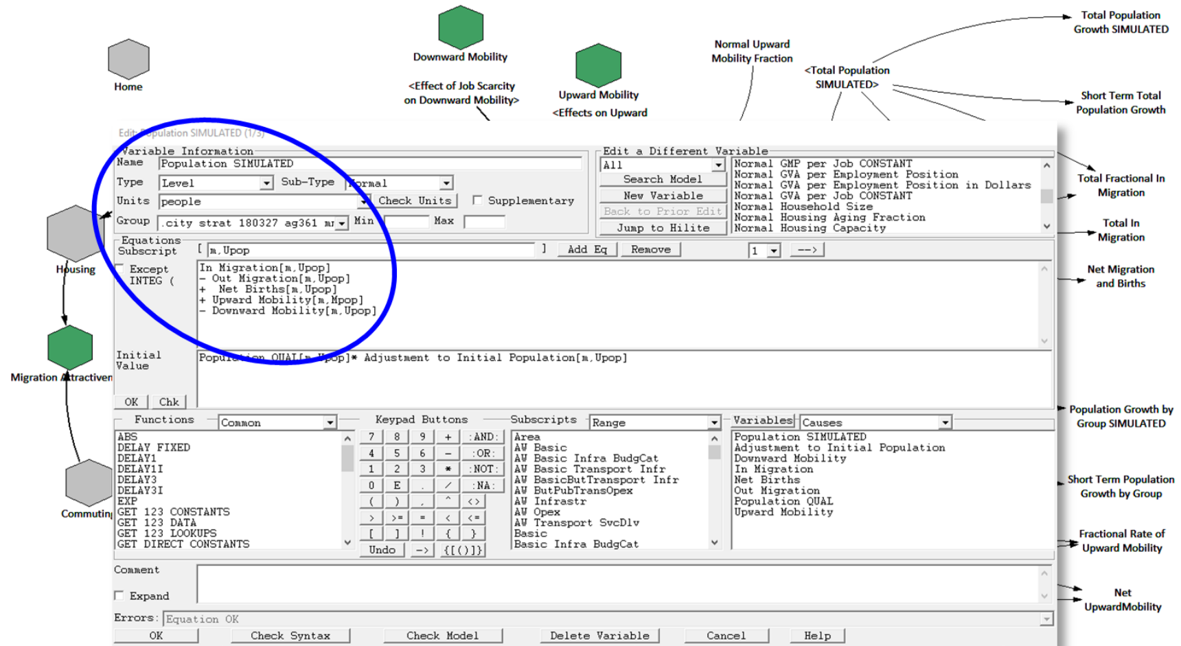
Figure 28 – Detailed equation level view of population
