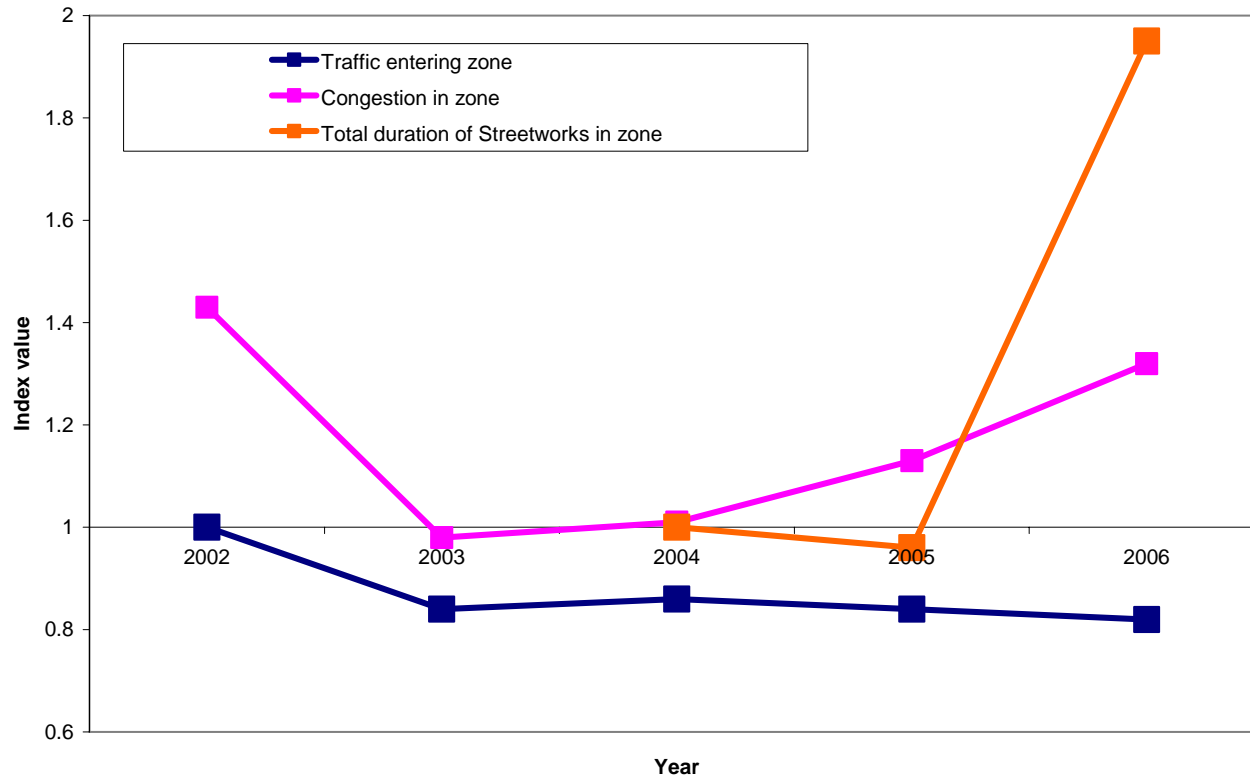
Delays, Streetworks Activity and Traffic Flows. Central London Congestion Charging Zone. 2002-2006.
